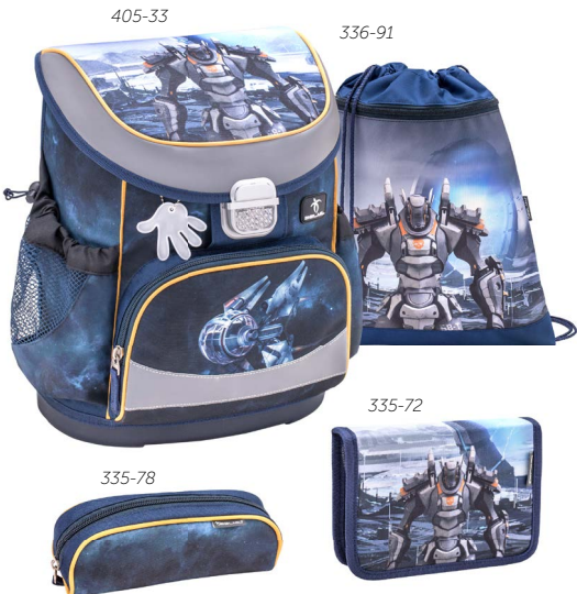
Parallel Universe
